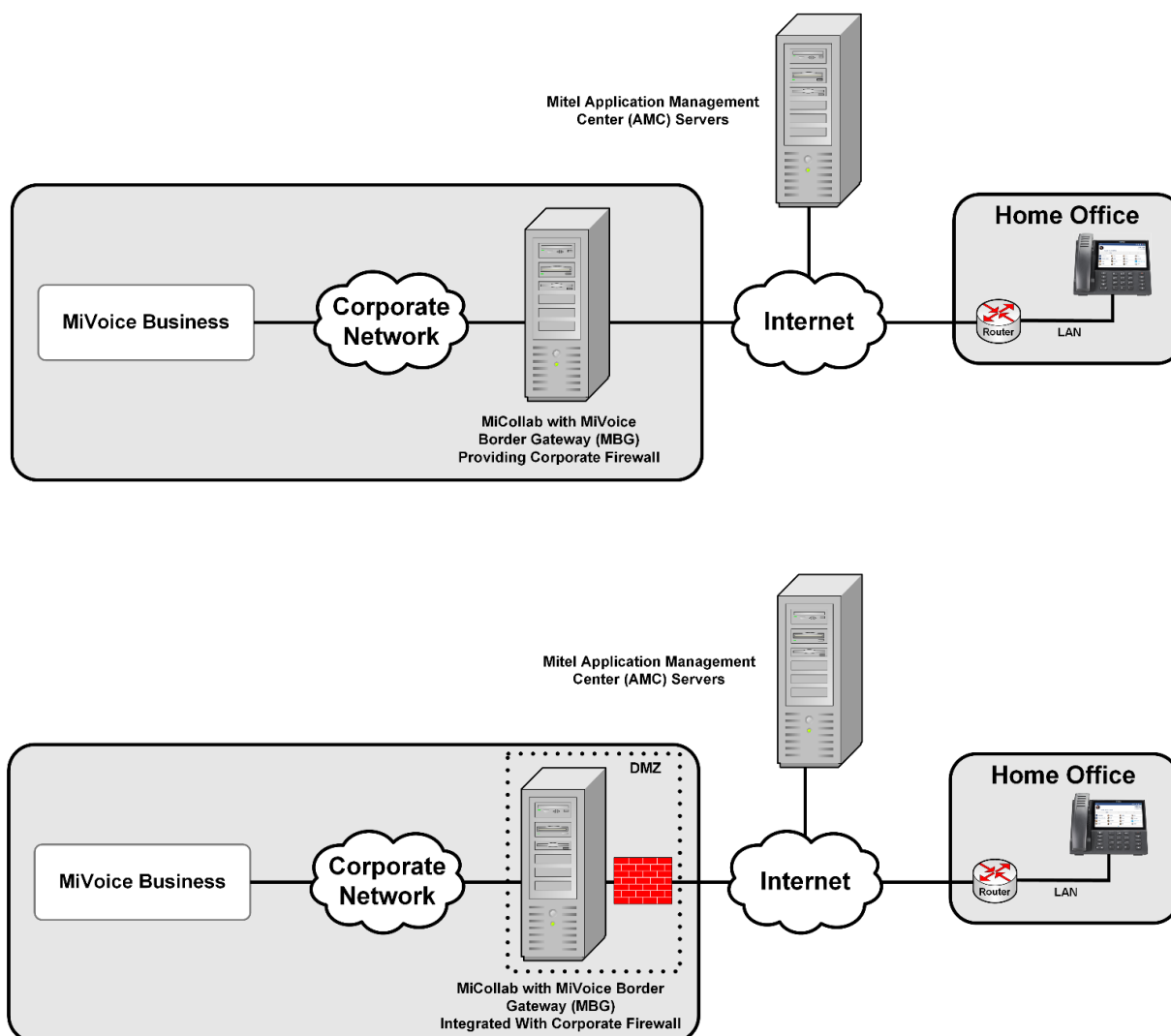
Figure 21: MiVoice Border Gateway Teleworker Service (Internet Facing and DMZ)
