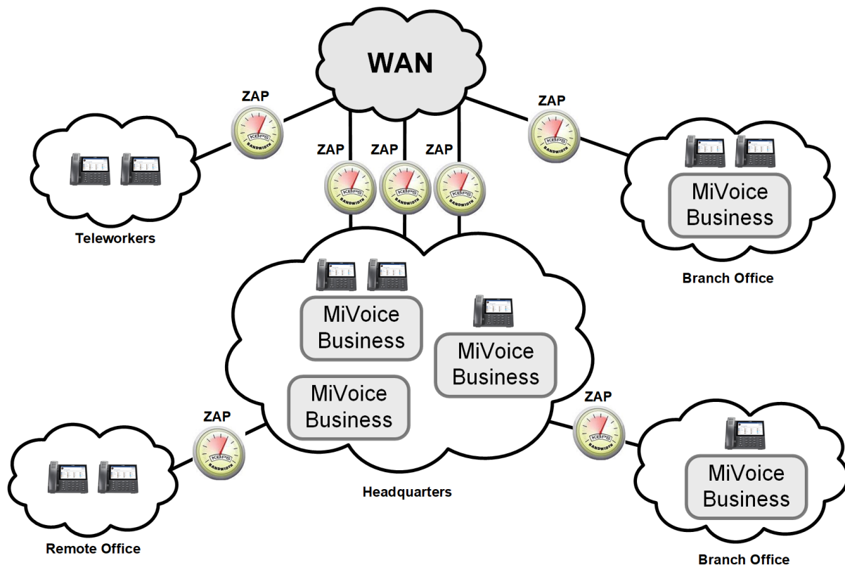
Figure 5: Example of Bandwidth Management Zone Access Points
