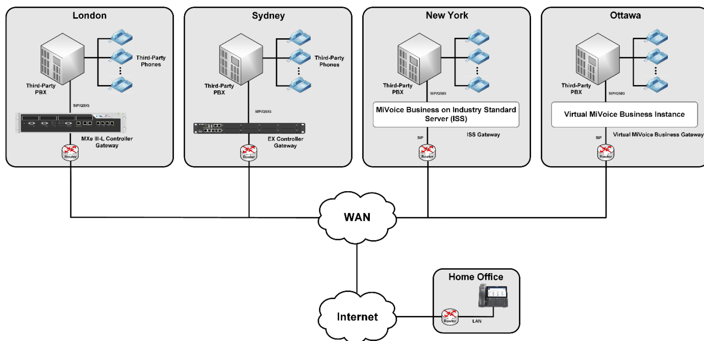
Figure 19: Example of MiVoice Business as Gateway
