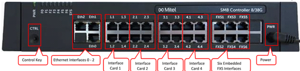
Figure 17: SMB Controller Front Panel
