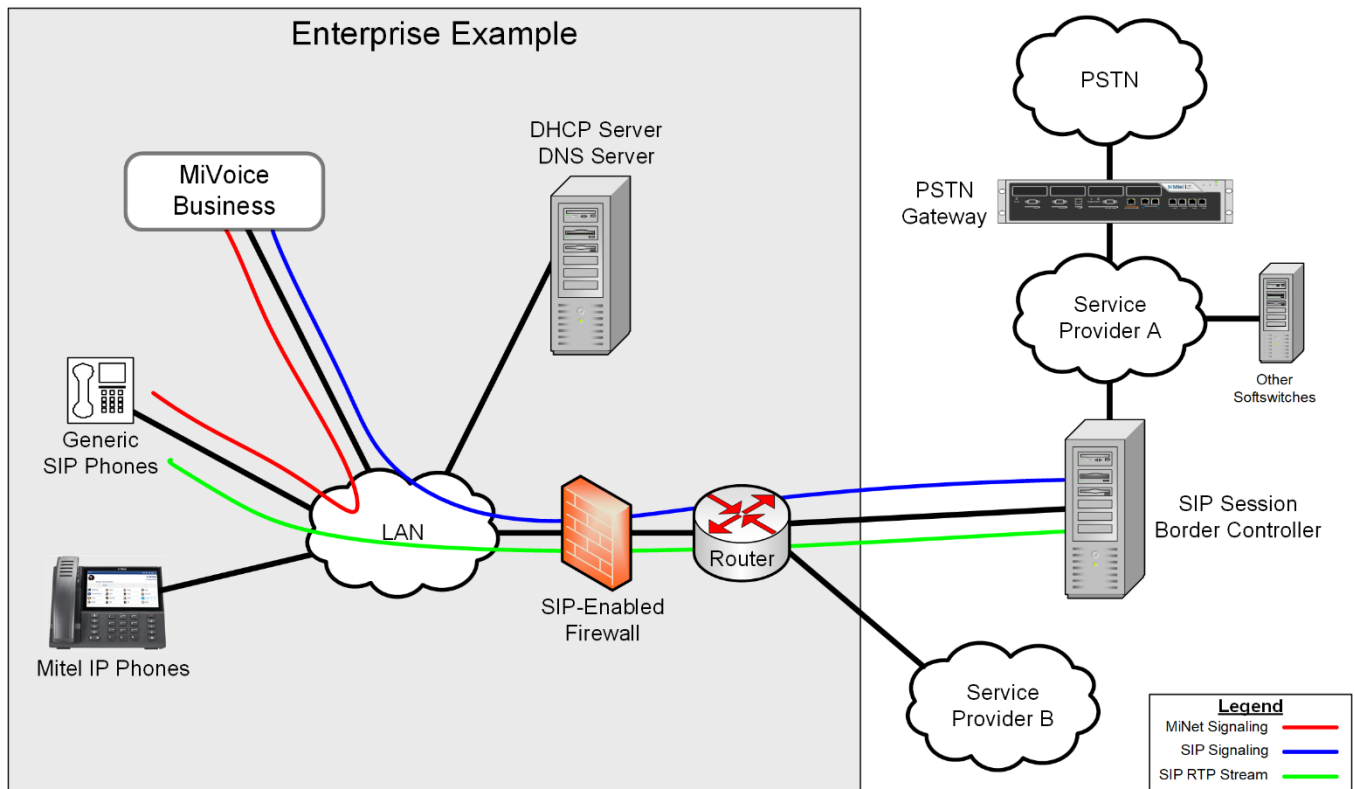
Figure 4: Example of a SIP Trunking Setup
