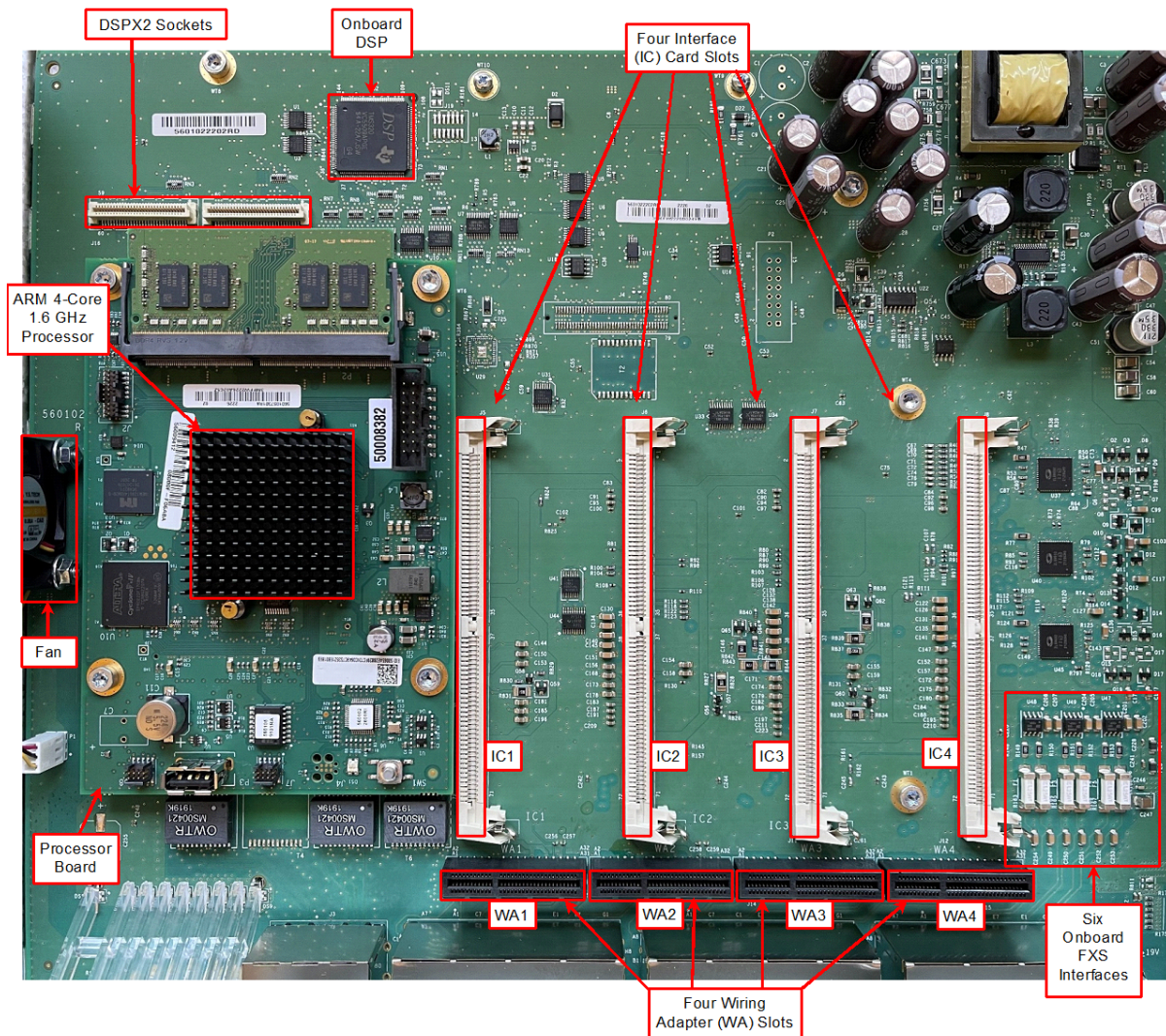
Figure 18: SMB Controller Internal
